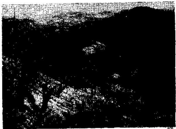
Fig. 4 The basin of fig. 2, seen in south westernly direction. k is limestone.
